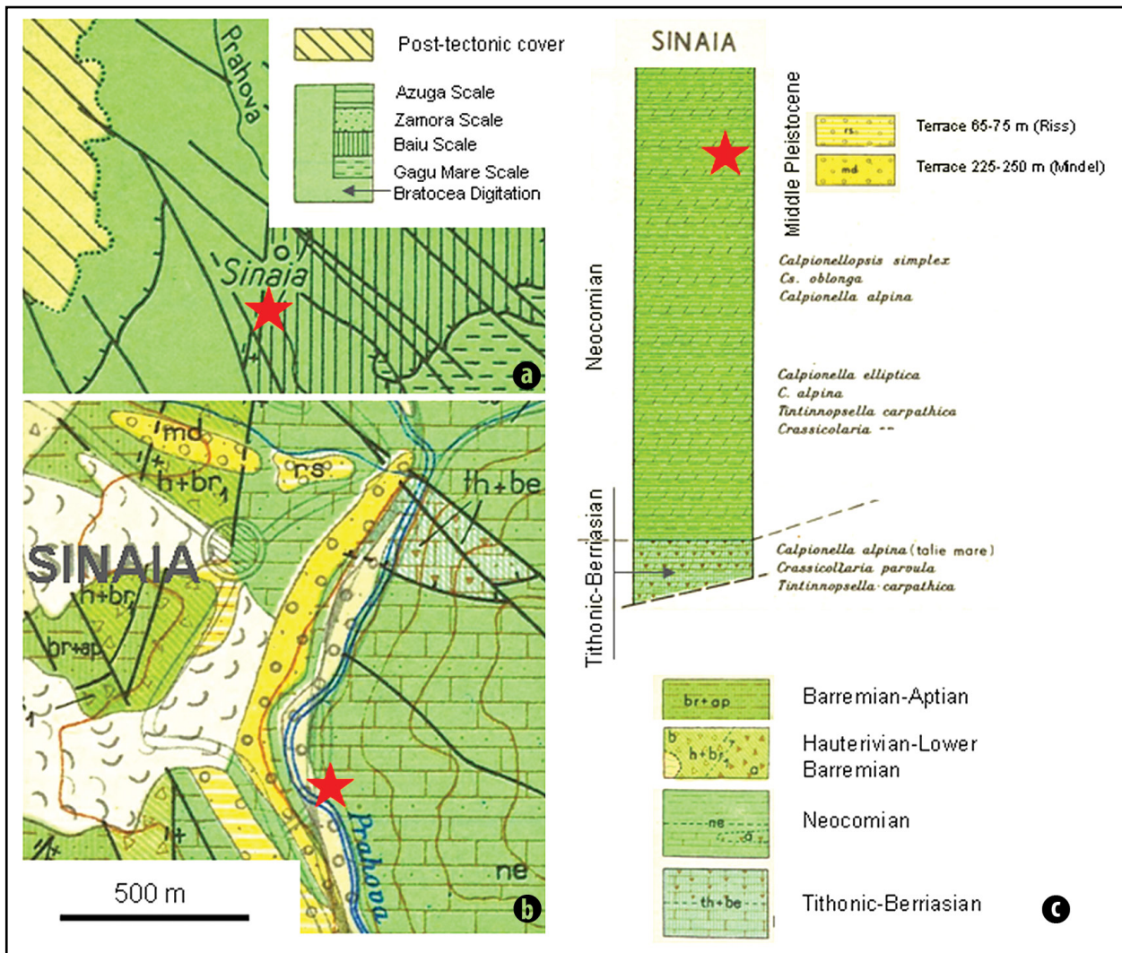
Fig. 1. Ichnofossiliferous site (red stars) location on the tectonic map (a), geological map (b) and lithostratigraphic column of the middle member of the Sinaia Formation (c) (simplified, acc. to Ștefănescu, 1980 – 111c Baiu sheet, scale 1: 50,000).
